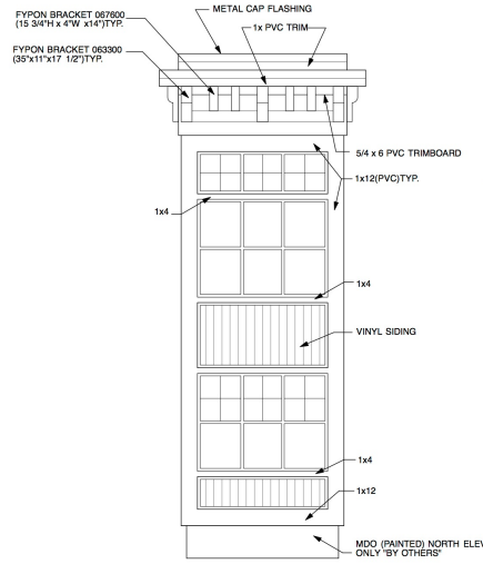
4 ENLARGED ELEV. BAY WINDOW (TYPE 1) SCALE: 1/4" = 1'-0"
