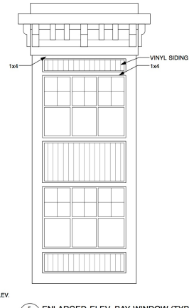
5 ENLARGED ELEV. BAY WINDOW (TYPE 2) SCALE: 1/4" = 1'-0"
