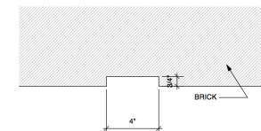
3 BRICK REVEAL DETAIL A-8 SCALE: 3/4" = 1'-0"
