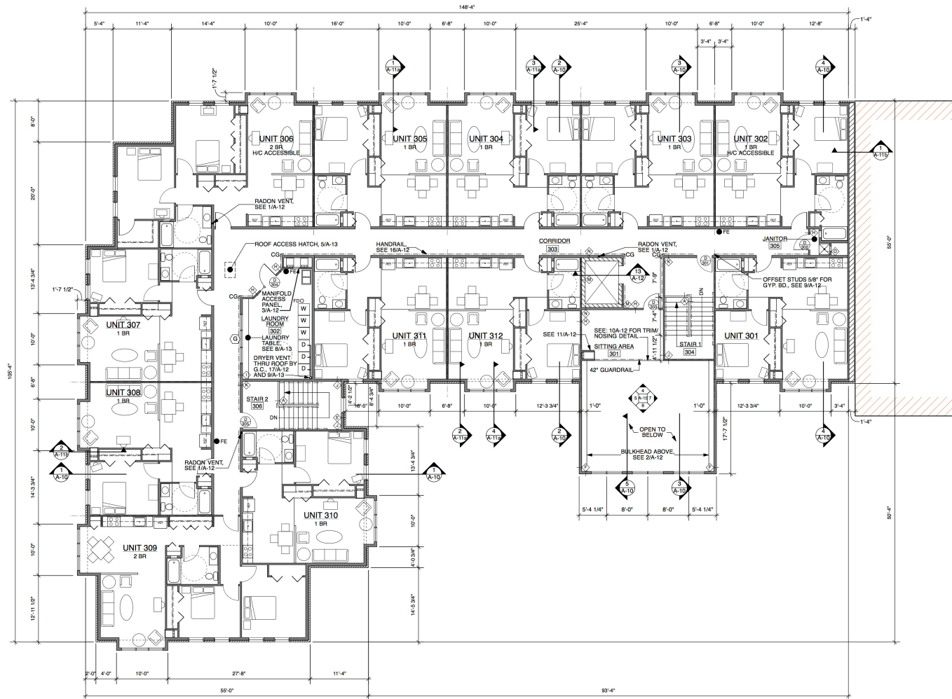
1 THIRD FLOOR PLAN A-5 SCALE: 1/8" = 1'-0"
