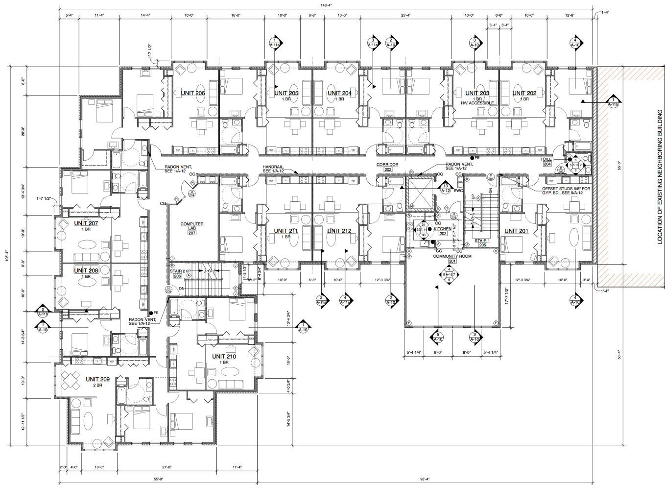
1 SECOND FLOOR PLAN A-4 SCALE: 1/8" = 1'-0"
